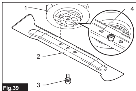
Fig. 39 ► 1. Blade support 2. Mower blade 3. Bolt 4. Protrusion
